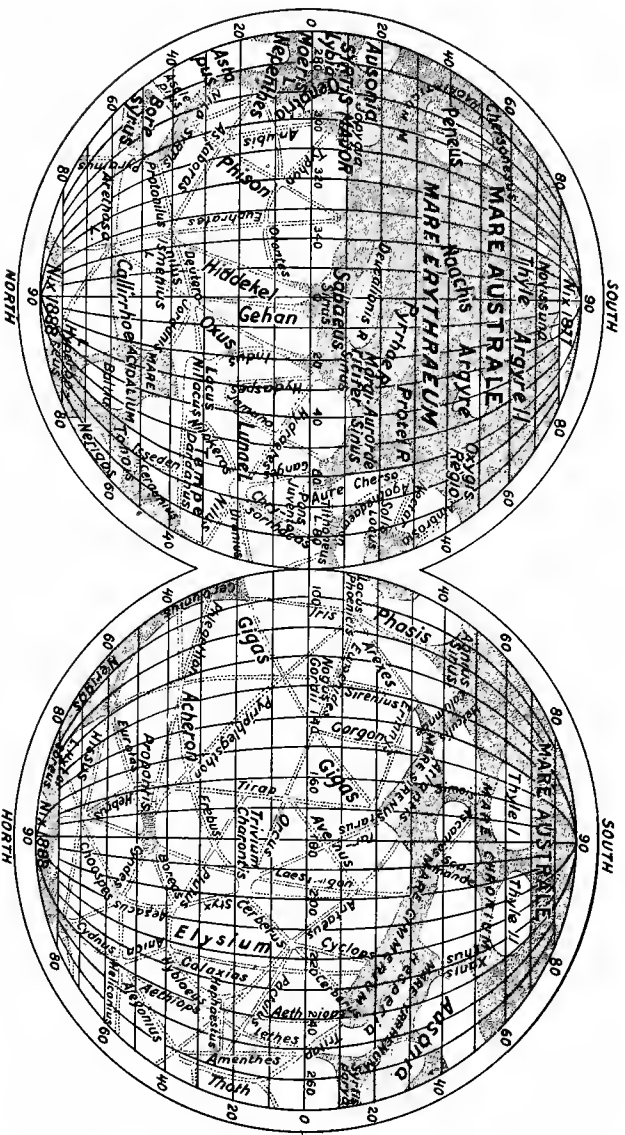
SCHIAPARELLI'S CHART OF MARS, SHOWING THE SYSTEM OF SO-CALLED CANALS
